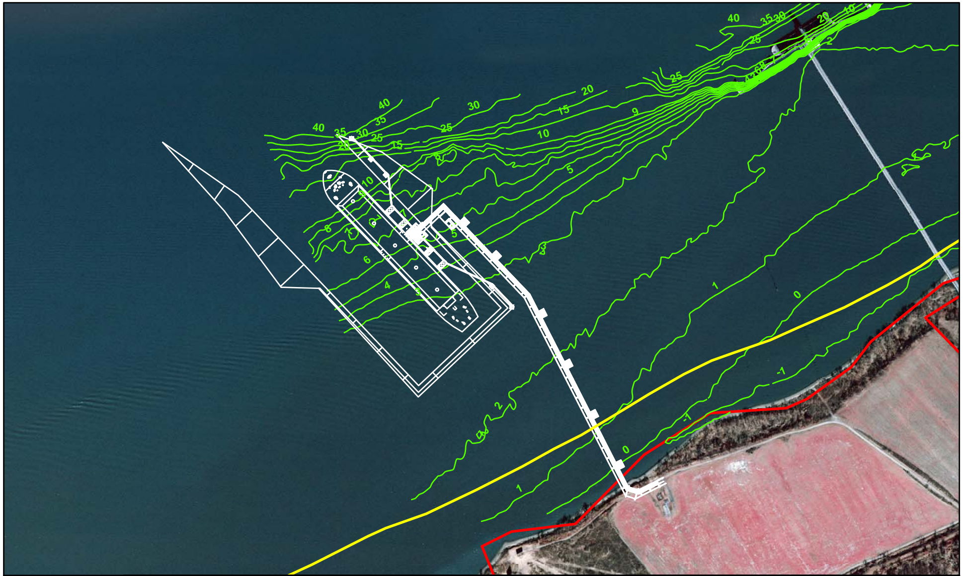
Figure 4 Berth and Dredged Area
